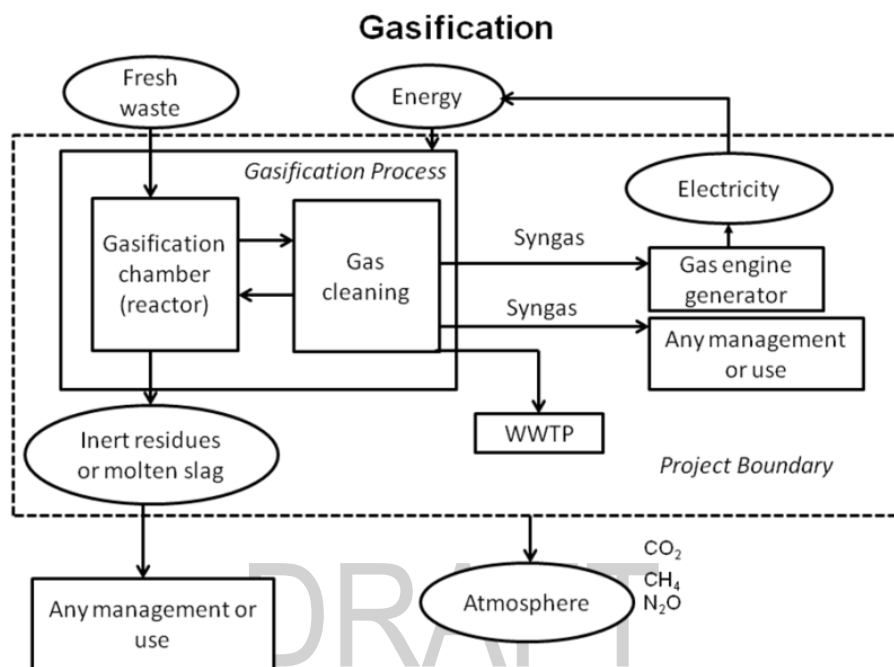
Figure 5. Gasification
