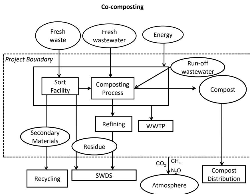
Figure 2. Co-composting
