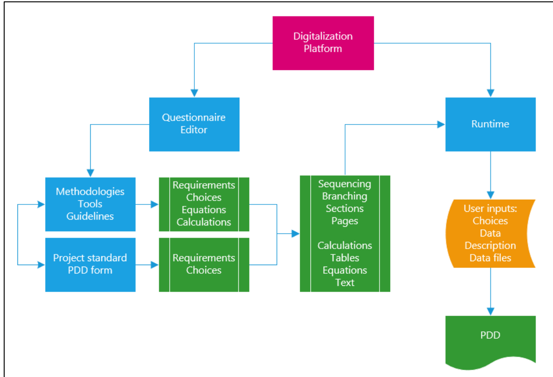
Figure 3. The system architecture of the digitalization platform
