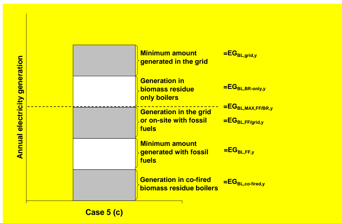
Figure 2. Determination of the baseline emission factor in case 5(c)
