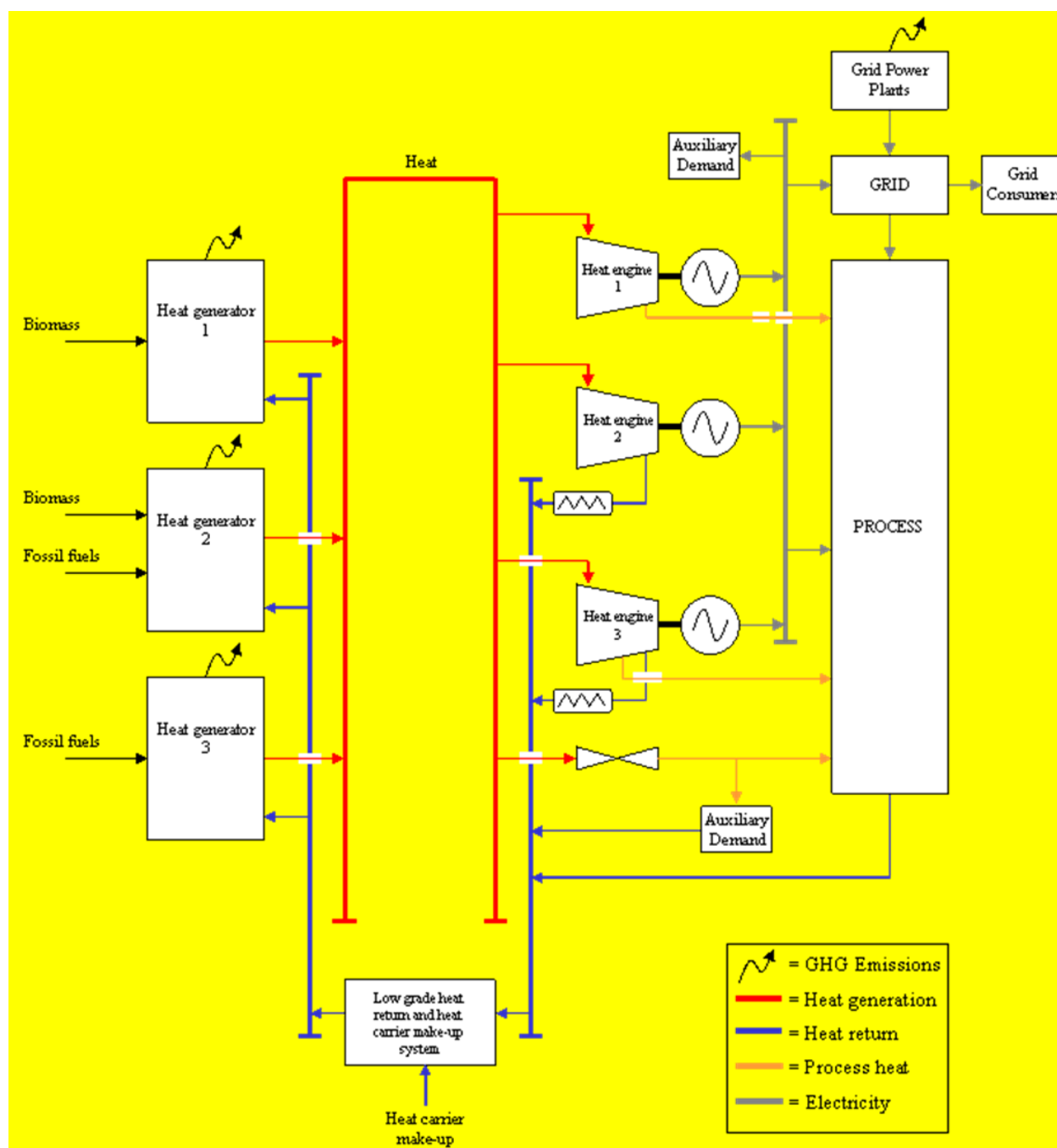
Figure 1. Schematic diagram of the CDM project activity and the baseline scenario 6
