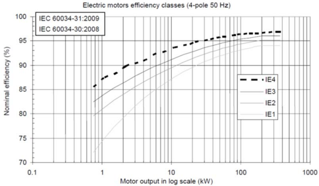
Figure 1. Efficiency classes of electric motors
