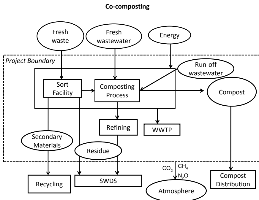
Figure 2. Co-composting
