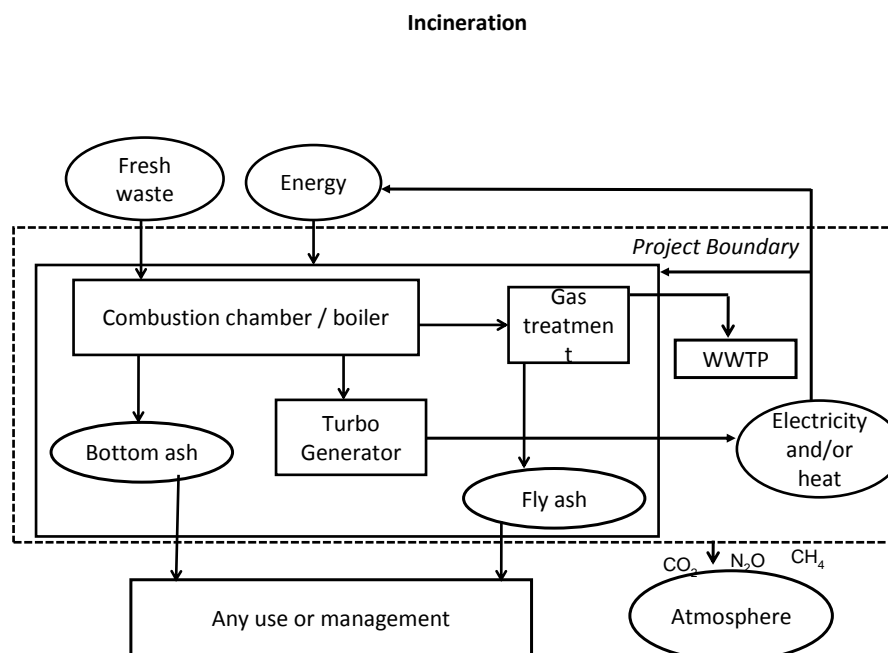
Figure 6. Incineration
