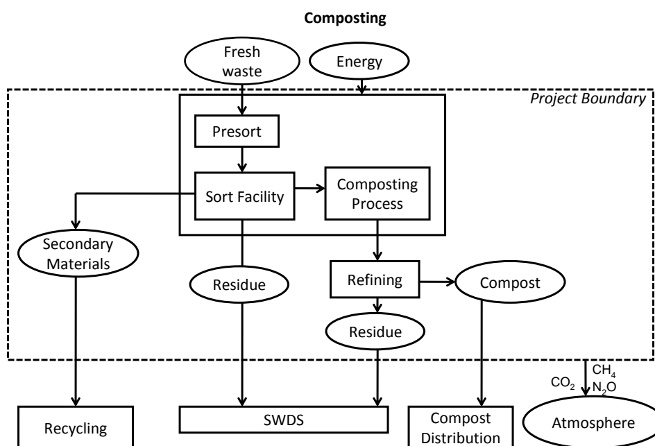
Figure 1. Composting
