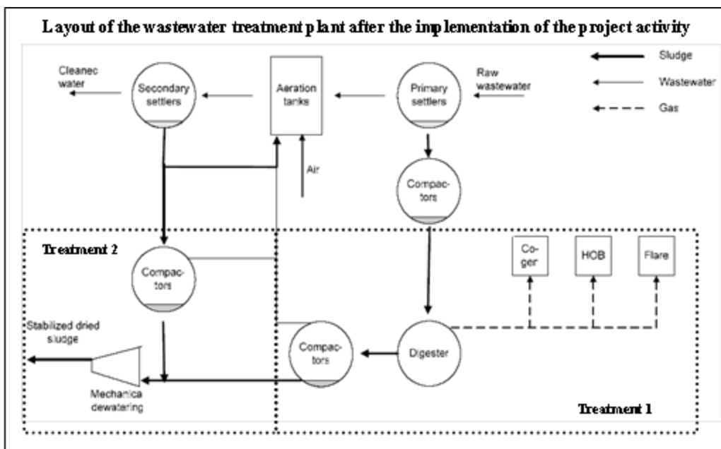
Figure 2. Layout of the project treatment plant
