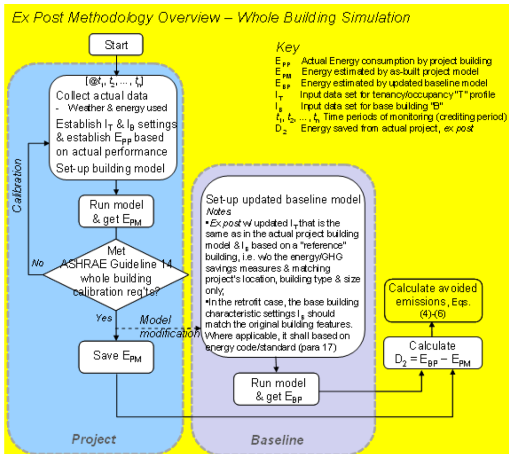
Figure 1. Flowchart of whole building simulation
