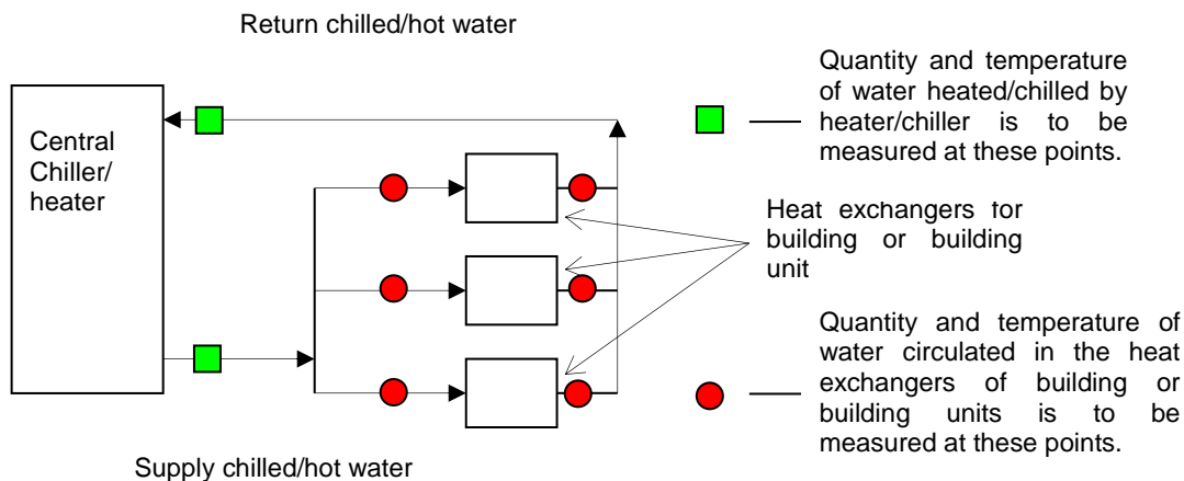
Figure 2. The applicable configuration of chilled/hot water system
