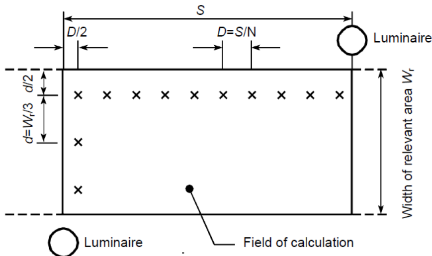
CIE 140:2000 Illustration of Illuminance Field of Calculation
