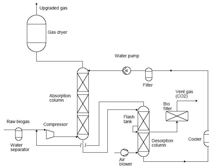
Figure 4: Absorption with water with recirculation 4
