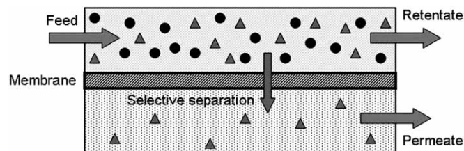
Figure 5: Schematic of membrane gas separation 5
