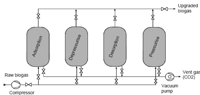
Figure 3: Pressure Swing Adsorption 3
