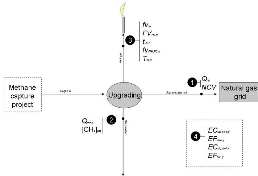
Figure 2: Monitoring system
