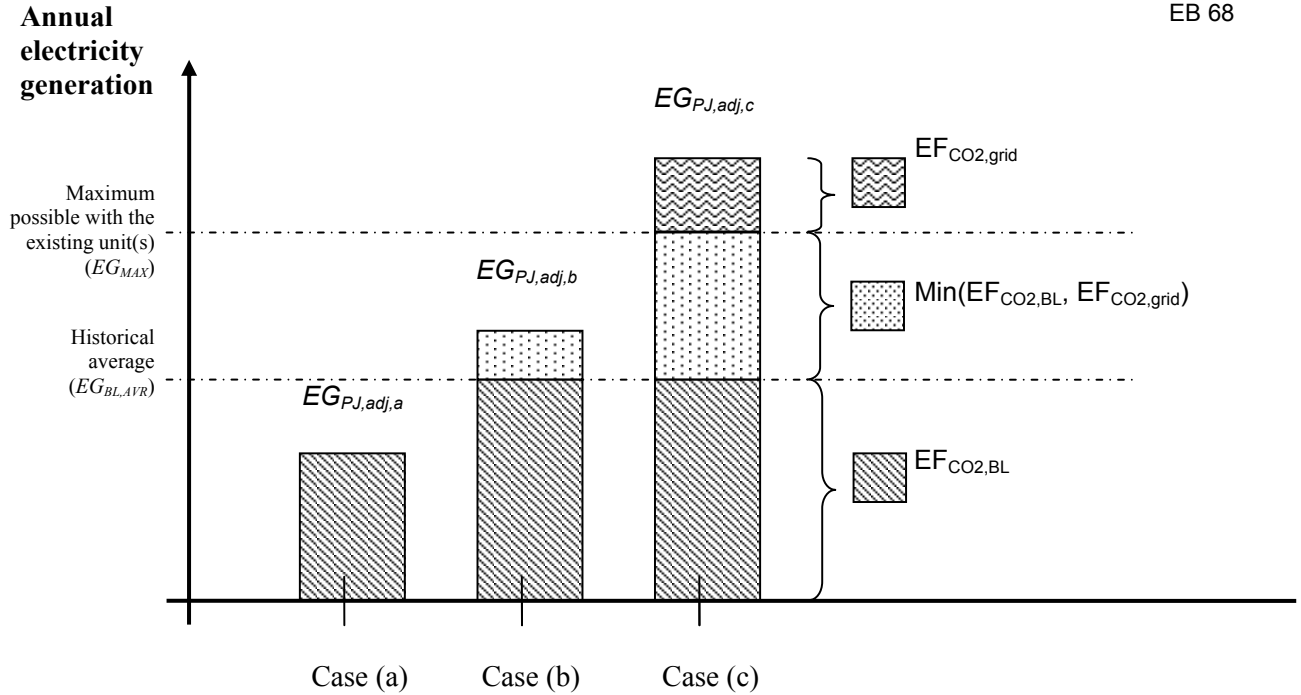
Figure 1: Baseline emissions calculation for three cases of different quantities of electricity generated
