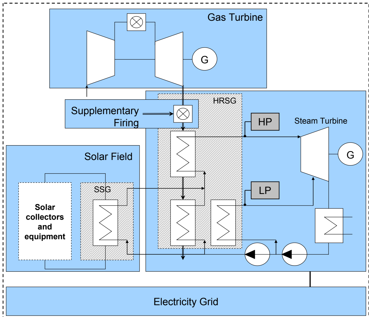
Figure 1: Simplified layout of an ISCC with illustration of the above definitions (project boundary illustrated as dotted line)
