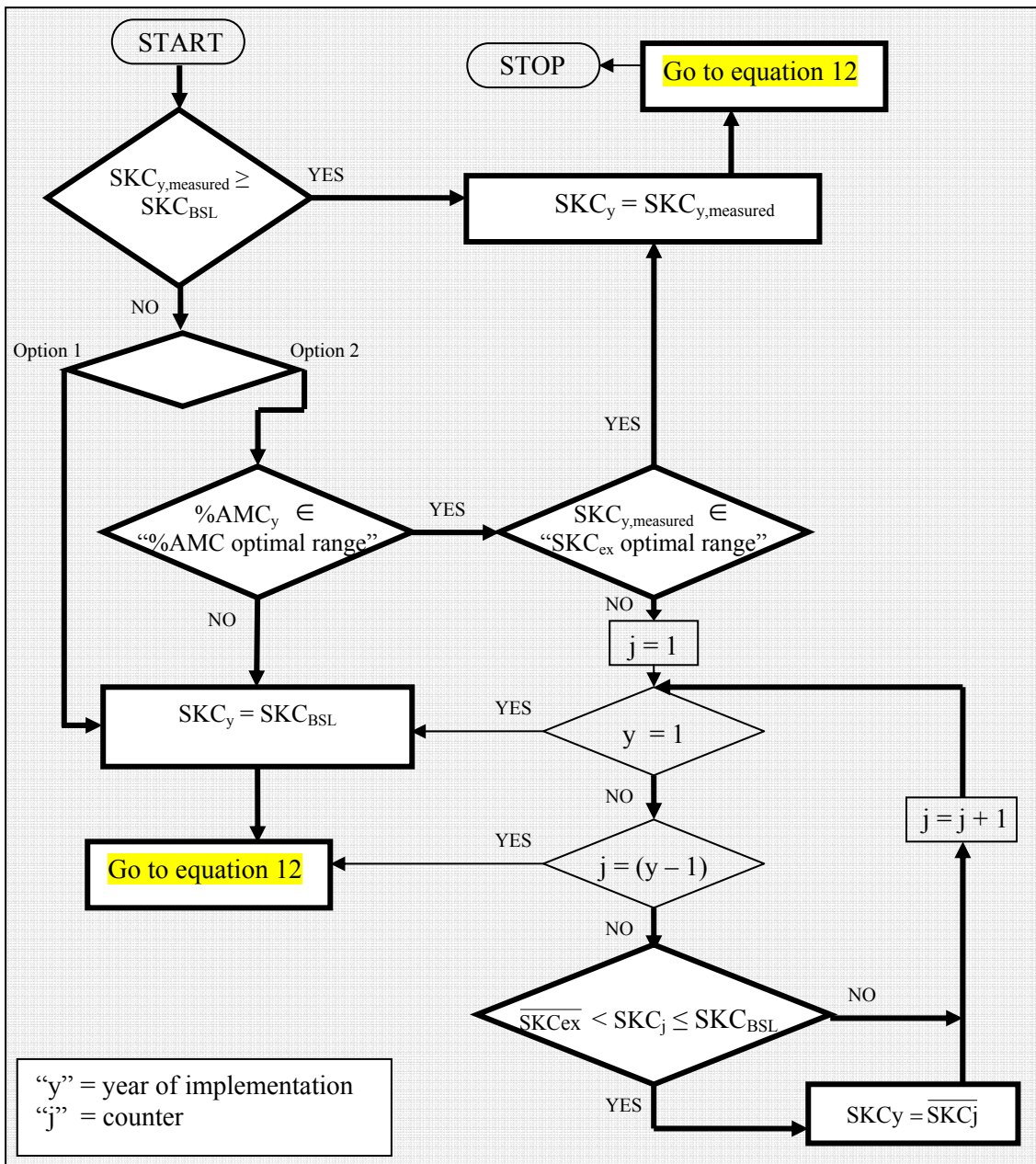
Diagram 1.1: “Flowchart of to assign value to SKC_y in equation 12 comparative procedure for Project Emissions in the year y ”
