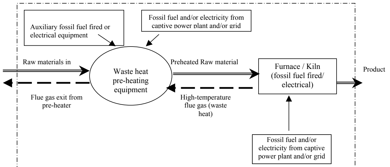
Figure 1: Schematic representation of the project boundary
