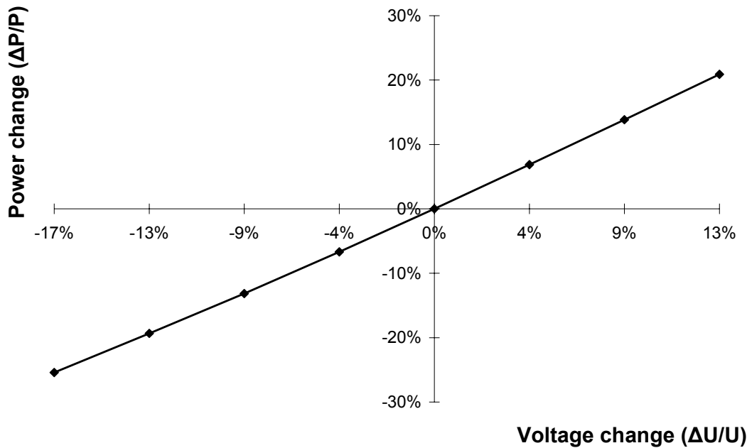
Figure 1: P-U characteristic curve for a 100 W incandescent lamp in a 230 V grid 9
