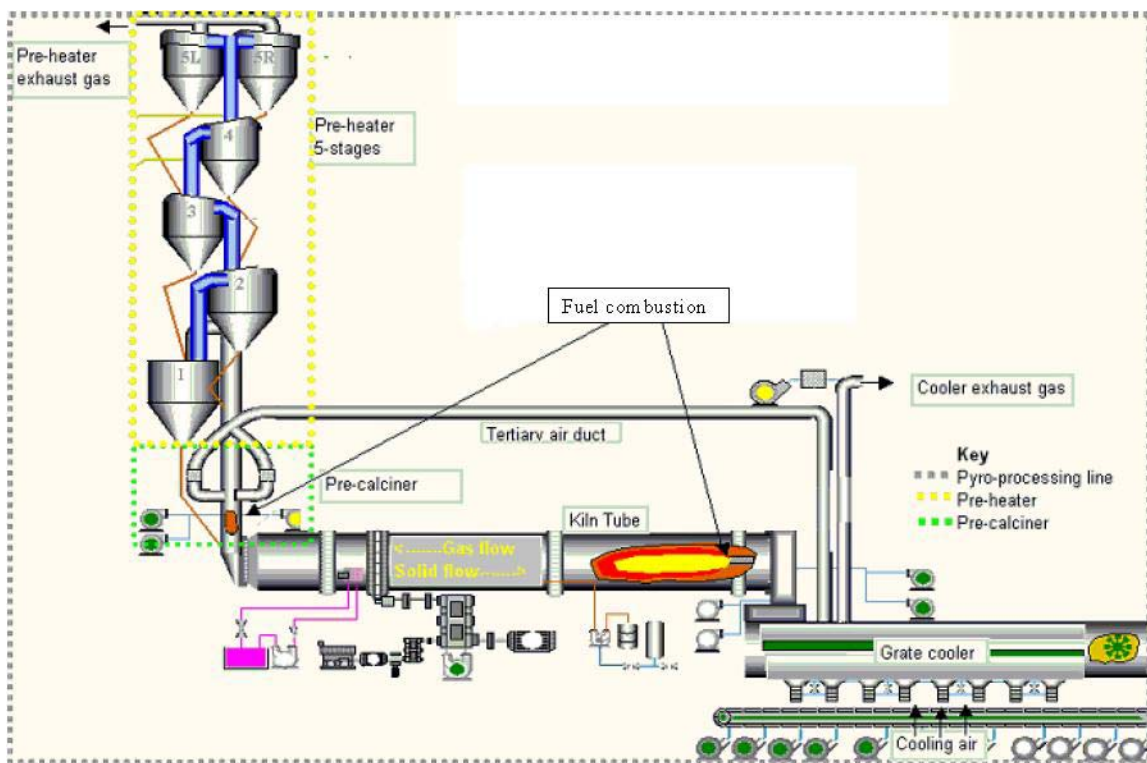
Figure 1 - Possible configuration of the pre-heaters, pre-calciner and kiln tube
