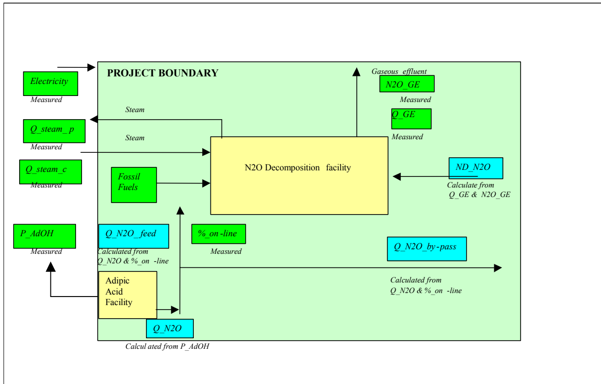
Figure 1: Schematic illustration of the project boundary
