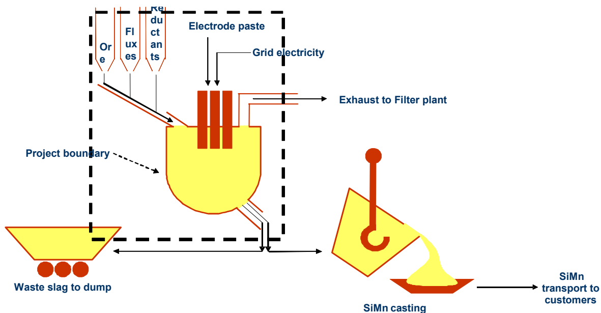
Figure 1: Spatial extent of the project boundary (excluding the grid generation capacity according to the latest version of ACM0002)
