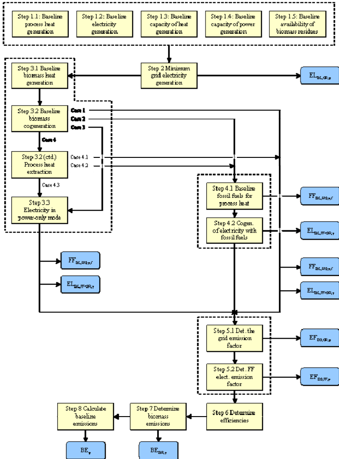
Figure 2 - Flow chart for the calculation of baseline emissions
