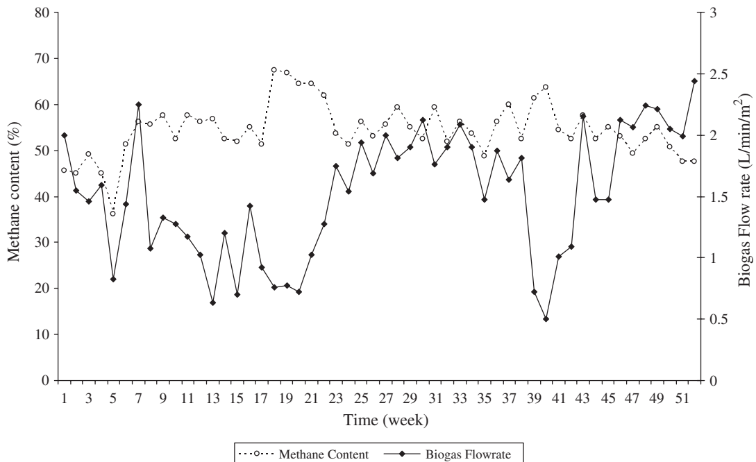
Fig. 2. Biogas emission profiles from anaerobic ponds.
