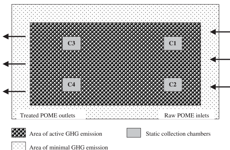
Fig. 1. Schematic top view diagram of anaerobic pond, areas of GHG emission, position of chambers and effluent flow.
