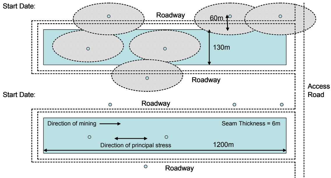
Figure 4. Indicative Figure Showing Mining Plan, relevant CBM wells and their zones of influence
