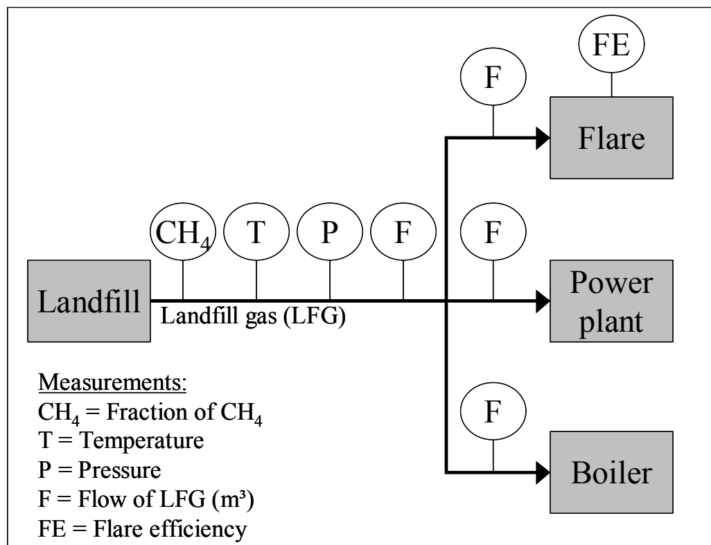
Figure 1: Monitoring Plan
